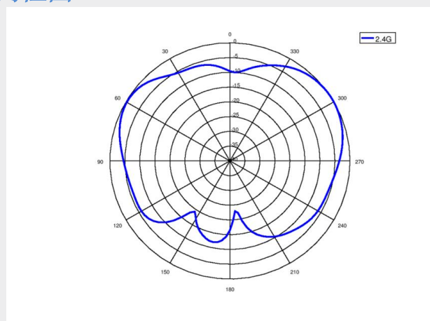
2.4G (PHI=90)
