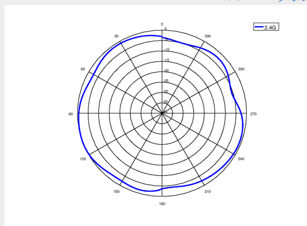
2.4G (PHI=0)
