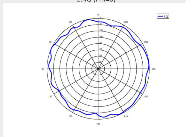
5G-1 (PHI=0)
