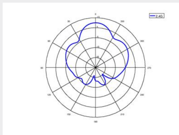
2.4G (PHI=90)
